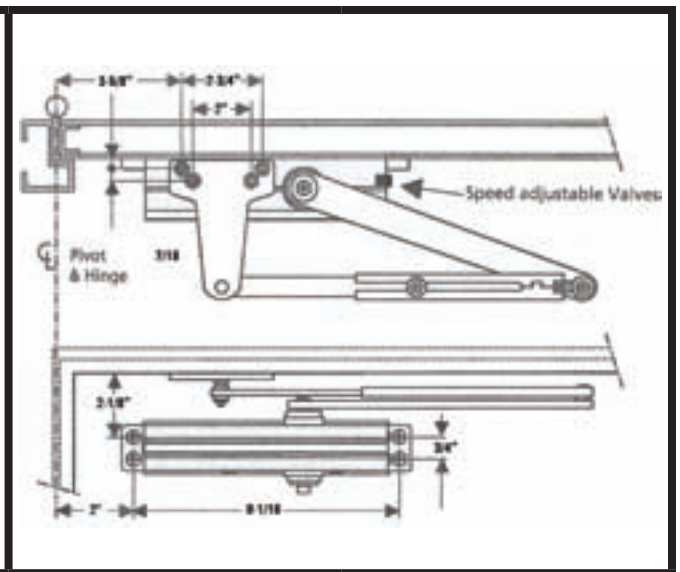
PUSH SIDE INSTALLATION
