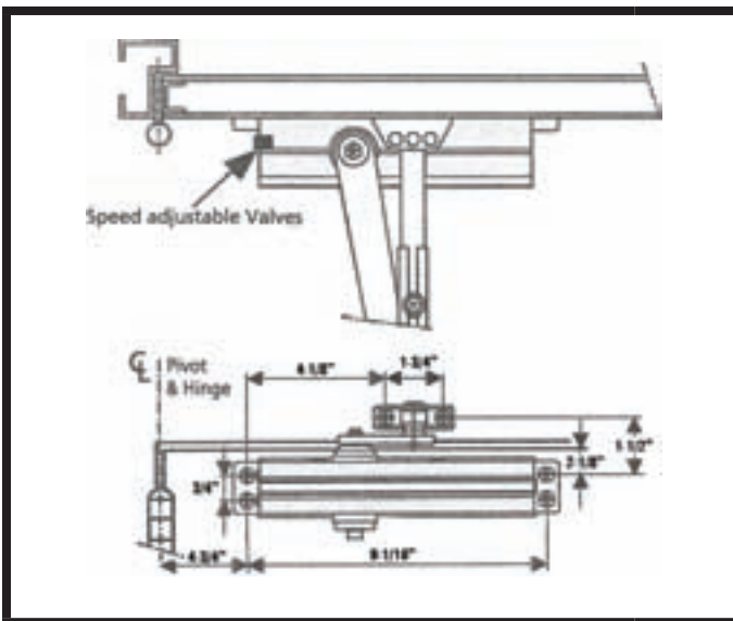
PULL SIDE INSTALLATION
