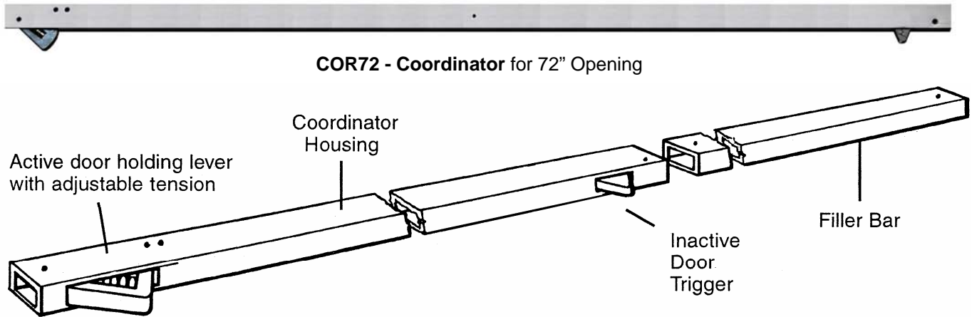
COR-72 – Coordinator for 72" Pair
